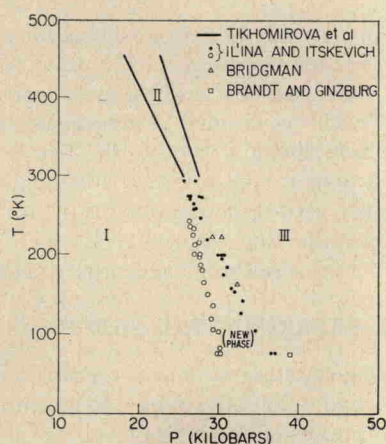
FIG. 1. The phase diagram of bismuth below room temperature. The open triangles refer to Bridgman's data (Ref. 1). The solid lines are straight lines drawn through the data of Tikhomirova et al. (Ref. 6). The open square is a point determined by Brandt and Ginzburg (Ref. 7). The circles represent a replotting of the data of Il'ina and Itskevich (Ref. 9).
